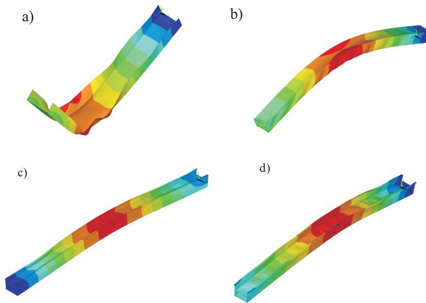
Figure 6 Dynamic response to impulse compression pressure of the profile with cross section: a) C channel, b) Rectangular, c) Internal tandem, d) External tandem
