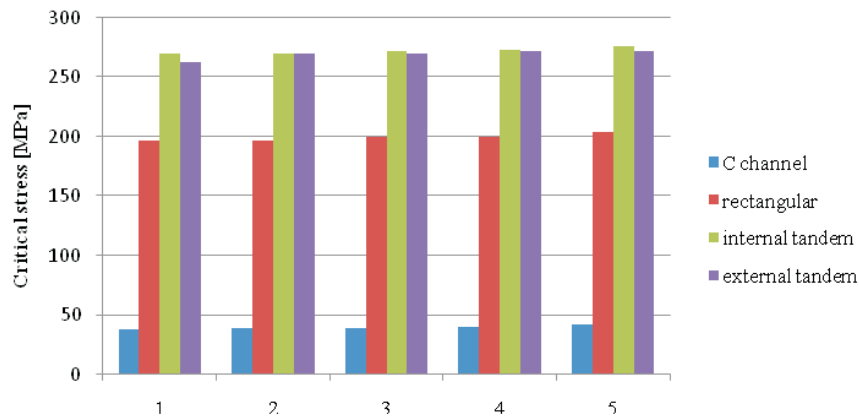
Figure 5 First 5 lowest values of critical stress for the axially compressed beams of different cross-sections
