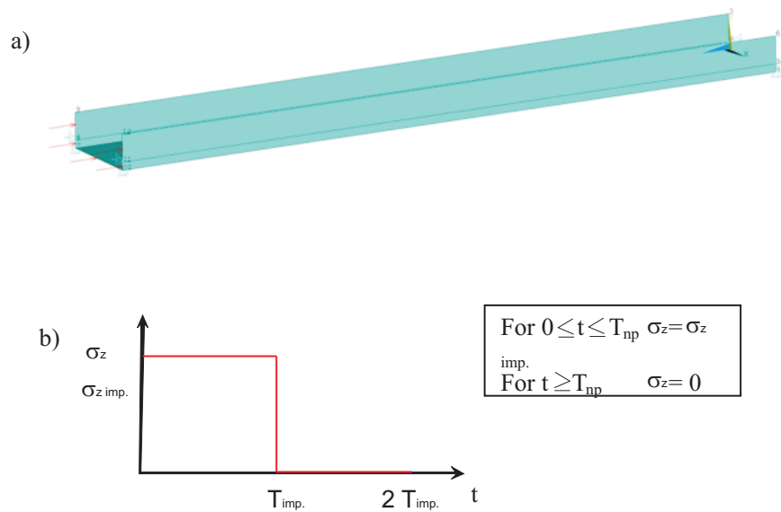
Figure 3 Loading details: a) C channel boundary conditions, b) The rectangular impulse loading characteristics
