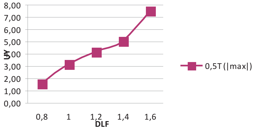
Figure 8 Dynamic deflection obtained with the FEM for Internal tandem- time duration of compression impulse equals 0.5 x natural period (of 1st mode)
