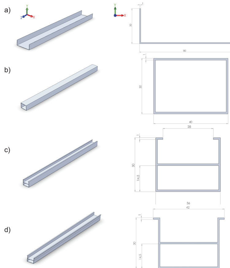
Figure 2 Considered cross-sections of the profile with dimensions: a) C channel, b) Rectangular, c) Internal tandem, d) External tandem
