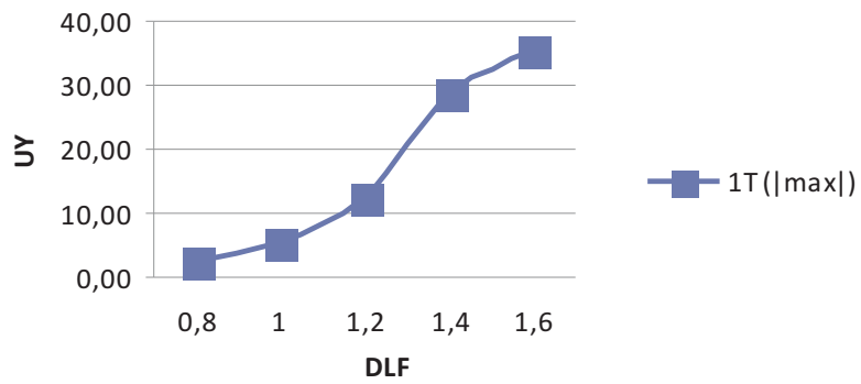
Figure 7 Dynamic deflection obtained with the FEM for Internal tandem- time duration of compression impulse equals 1 x natural period (of 1st mode)
