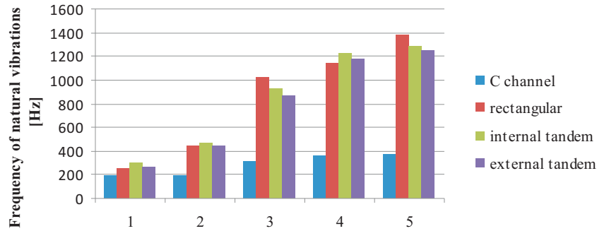
Figure 4 First 5 lowest natural frequencies for the beams of different cross-sections
