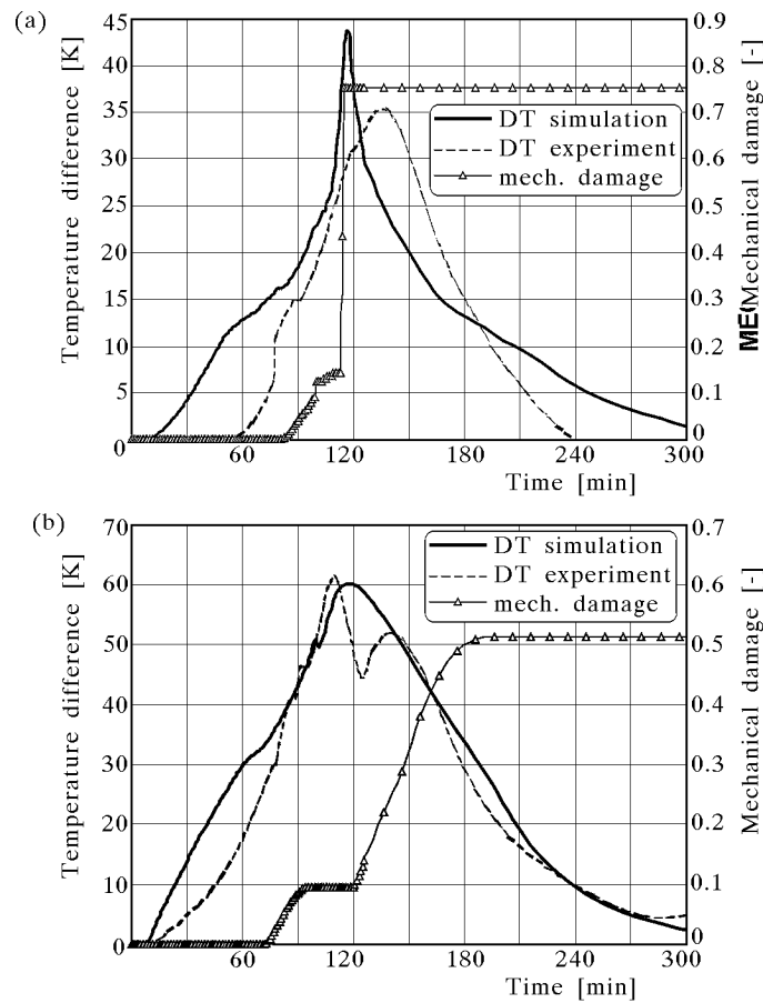
Fig. 1. Time evolution of the mechanical damage parameter and temperature difference in concrete specimens made of two types of the concrete: (a) MIX-1, (b) MIX-2, in a NIST experimental test
