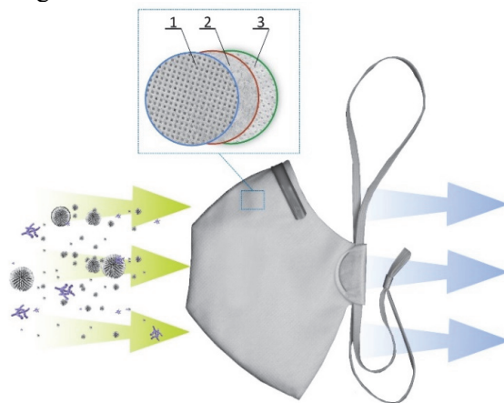
Figure 1. Arrangement of filtering layers in the construction of the bioactive half mask: 1) spun-bonded nonwoven ( 90 \text{ g/m}^2 ), 2) electret PP melt-blown nonwoven with SPBS ( 120 \text{ g/m}^2 ), 3) spun-bonded nonwoven ( 40 \text{ g/m}^2 )
