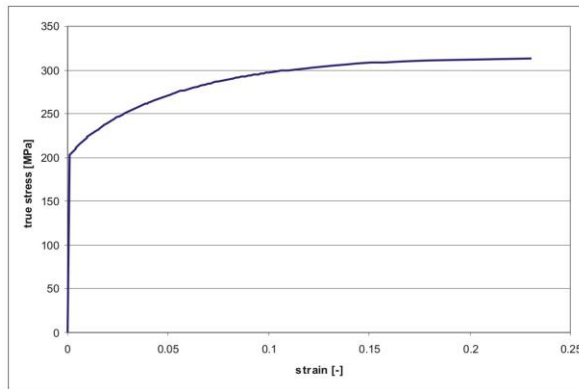
Fig.4. Material stress-strain relation obtained in laboratory for steel in tensile test
