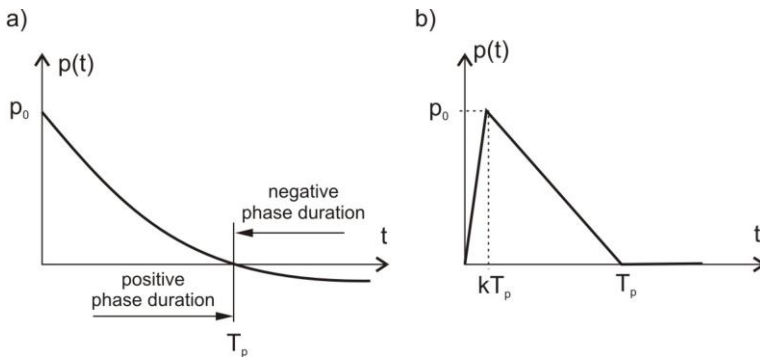
Fig.1. Blast pressure representation a) empirical b) triangular approximation
