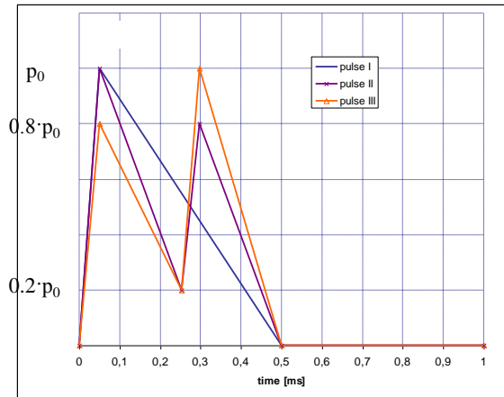
Fig.2. Assumed simulations of reflected blast pressure [4]
