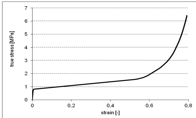
Fig.5. Material stress-strain relation obtained in laboratory for aluminium foam in compression test
