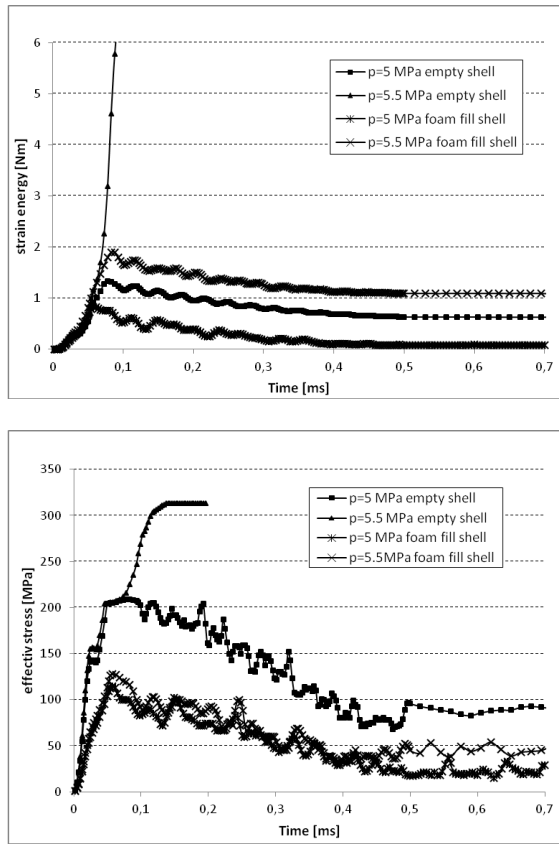
Fig. 6. Strain energy a) and effective stress b) time relations for steel shell and for foam filled shell subjected to pulse I (see Fig. 2)
