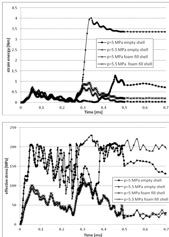
Fig. 8. Strain energy and effective stress time relations for steel shell and for foam filled shell subjected to pulse III (see Fig. 2)
