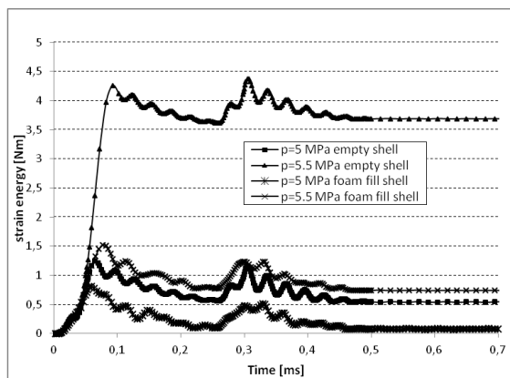
Fig. 7a. Strain energy time relations for steel shell and for foam filled shell subjected to pulse II (see Fig. 2)
