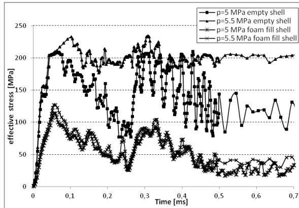
Fig. 7b. Effective stress time relations for steel shell and for foam filled shell subjected to pulse II (see Fig. 2)
