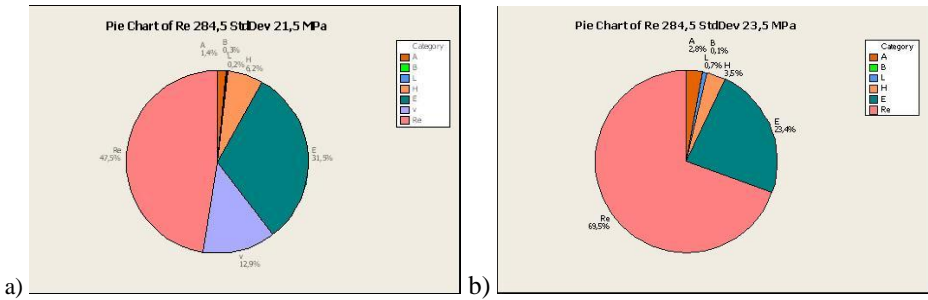
Fig. 4. Exemplary pie charts (UBELC sensitivity analysis – yield stress variance): a) 21.5 MPa standard deviation, b) 23.5 MPa standard deviation
