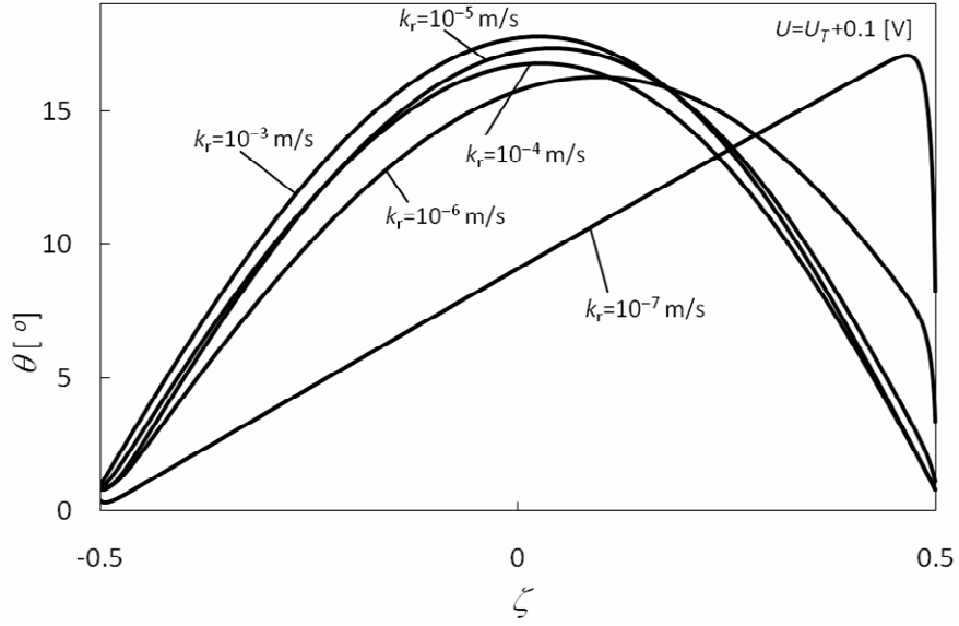
Fig. 4. Director profiles \theta as a function of the reduced coordinate \zeta for high ion concentrations. k_r in \text{ms}^{-1} are indicated at each curve
