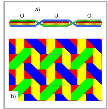
Figure 4. a) Diagram of tape interlacing, b) schematic view of a four-axial NP fabric [13].
