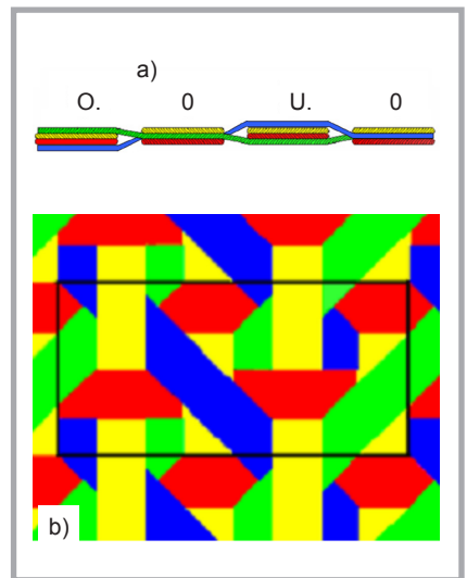
Figure 5. a) Diagram of tape interlacing, b) schematic view of a four-axial NO/PO fabric [13].
