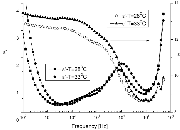
Fig. 1. Dielectric spectrum of the investigated mixture at chosen temperatures for two relaxation modes in the ferroelectric phase
