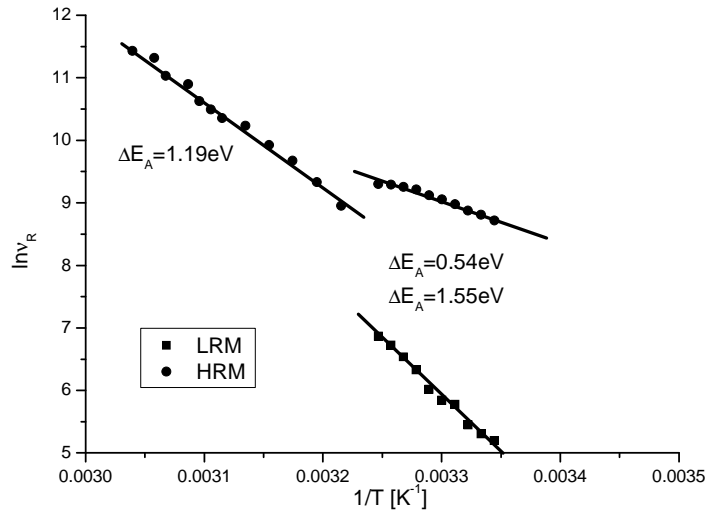
Fig. 7. Arrhenius plots for the relaxation processes in the ferroelectric phase
