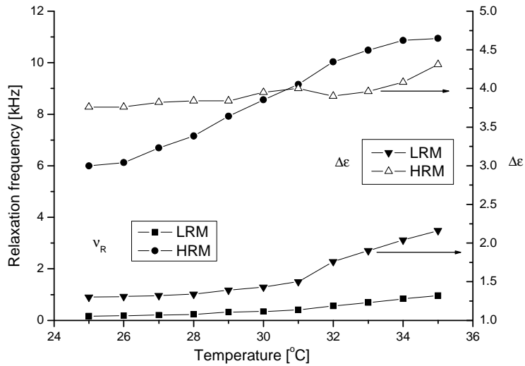
Fig. 4. Temperature dependence of the relaxation frequencies and the dielectric strength of ferrielectric phase
