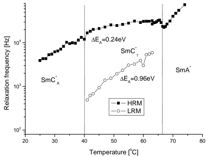
Fig. 9. Temperature dependence of relaxation frequency in the mixture (5:5) investigated earlier [11]
