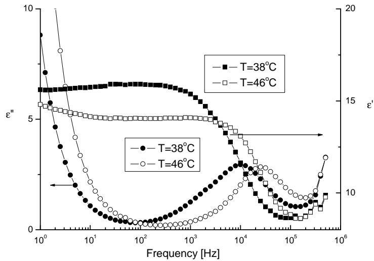
Fig. 2. Dielectric spectrum in higher temperature range of ferroelectric phase
