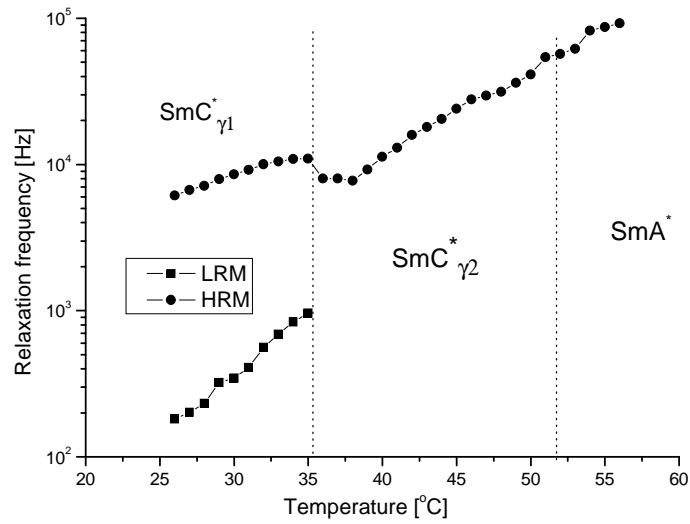
Fig. 5. Temperature dependence of the relaxation frequency in the ferroelectric and \text{SmA}^* phases
