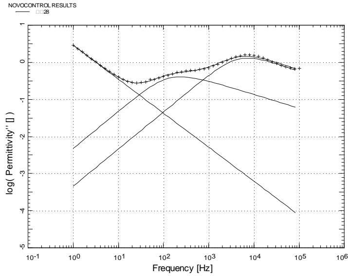
Fig. 3. Fitting procedure to Havriliak-Negami equation for two peaks observed in the ferrielectric phase
