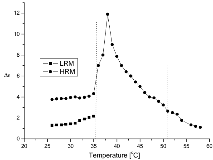
Fig. 6. Temperature dependence of the dielectric strength in the ferroelectric and \text{SmA}^* phases
