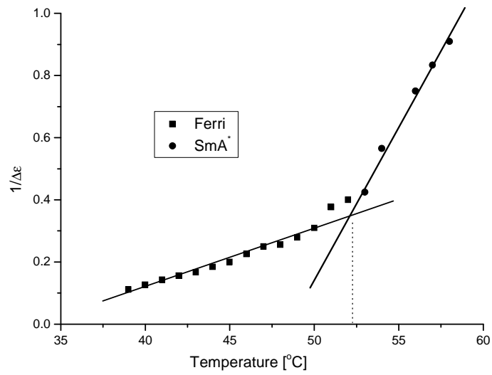
Fig. 8. Temperature dependence of the inverse of the dielectric strength in the SmA* and the ferrielectric phases
