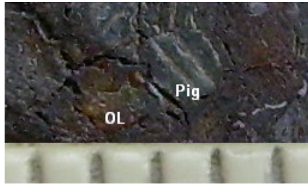
Fig. 3. Optical image of Shisr 007 showing olivine (OL) and pigeonite (Pig)
