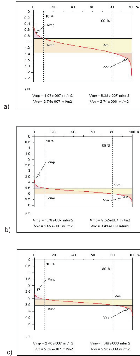
Figure 9 The volumetric functional parameters of the grinded surface:a) Brinnar 400, b) Dildur 500V, c) XAR 400
