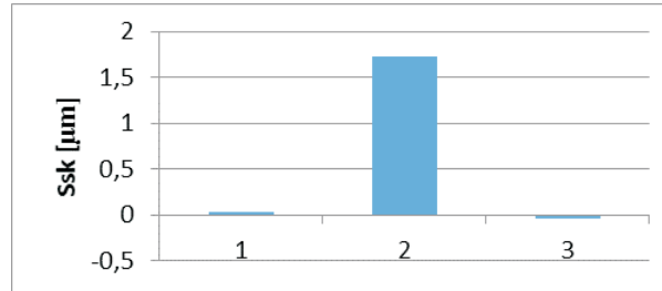
Figure 7 The value of the surface skewness Ssk: 1 – Brinnar 400, 2 – Dillidur 500V, 3 – Xar 400
