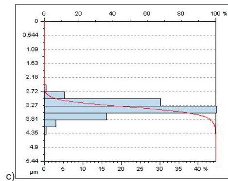
Figure 8 The shape of the curves participation of the material and distribution of ADF functions of the surface: a) Brinnar 400, b) Dilidur 500V, c) XAR 400
