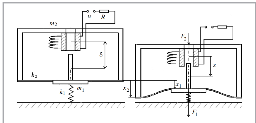
Figure 1. Schematic diagram of an elastic system resting on a textile layer and subjected to an electromagnetic oscillating force.
