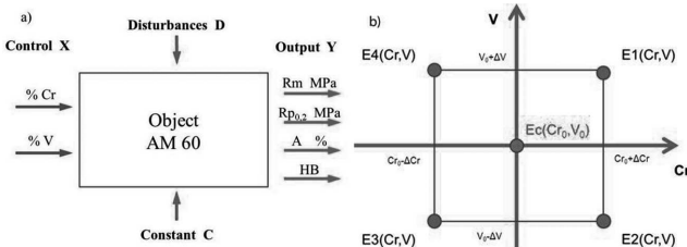
Fig. 1. Discussed non-linear object in the planned experiment for AM60 magnesium alloys (a), experiment plan for AM60 magnesium alloys with Cr and V additions (b)
