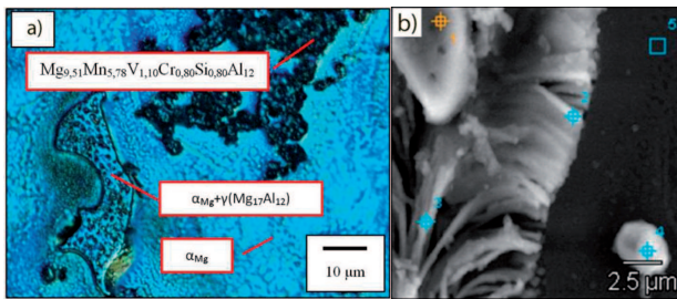
Fig. 4. Microstructure of AM60+0.1% V+0.1% Cr alloy solidifying in a ceramic mold observed by means of optic microscope (a) and scanning microscope (b)
